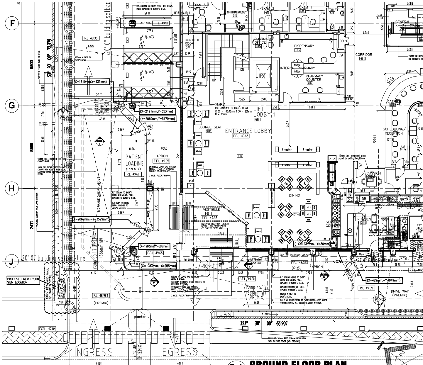
Grd. GROUND FLOOR PLAN 02-02 SETAPAK HOSPITAL SCALE 1: 100
